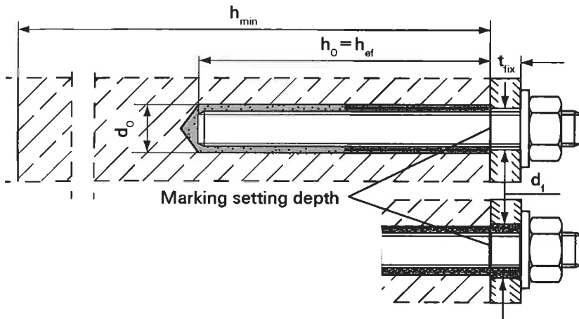
fischer anchor rod Pre-positioned anchorage
